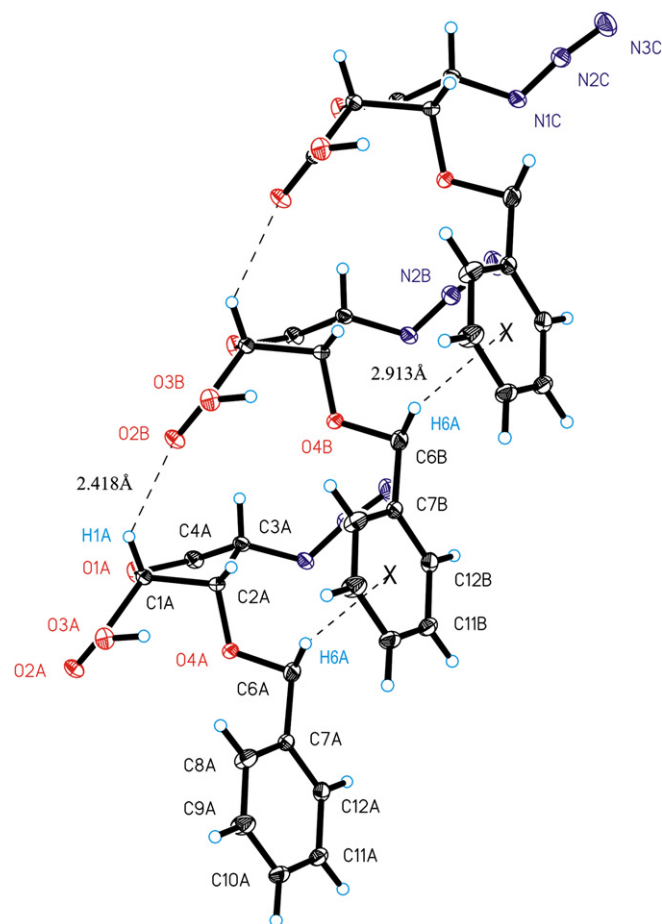
Figure 3. The partial crystal-packing of the SAA 8 showing the weak intermolecular C–H \cdots O and C–H \cdots\pi interactions. Few H-atoms have been omitted for clarity.
