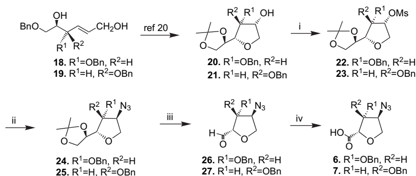
Scheme 3. Reagents and conditions: (i) MsCl, Et 3 N, CH 2 Cl 2 , 0 °C → rt, 30 min; (ii) NaN 3 , Bu 4 NCl (cat), DMF, 120 °C, 10 h for 24 (62% from 20 ), and 3 h for 25 (90% from 21 ); (iii) H 5 IO 6 (1.3 equiv), EtOAc, 30 min; (iv) Jones reagent, acetone, 0 °C, 10 min, 64% for 6 from 24 , 60% for 7 from 25 .
