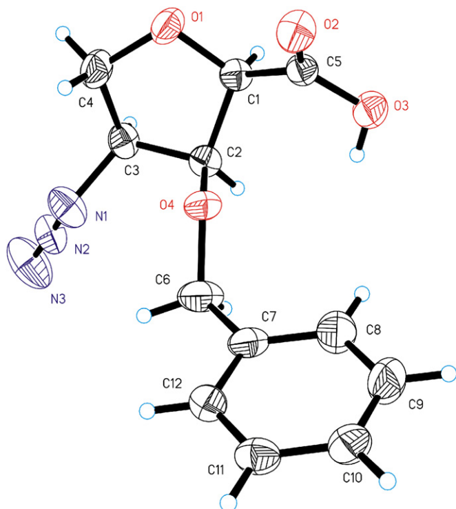
Figure 2. ORTEP plot of the SAA 8 (at 30% probability) showing the molecular conformation.
