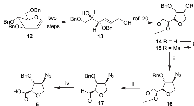
Scheme 2. Reagents and conditions: (i) MsCl, Et 3 N, CH 2 Cl 2 , 0 °C → rt, 30 min; (ii) NaN 3 , Bu 4 NCl (cat), DMF, 120 °C, 3 h, 90% (for two steps); (iii) H 5 IO 6 (1.3 equiv), EtOAc, rt, 30 min; (vi) Jones reagent, acetone, 0 °C, 10 min, 60% (for two steps).
