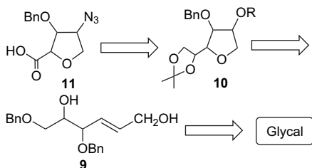
Scheme 1. General strategy followed for the synthesis of furanoid SAAs.
